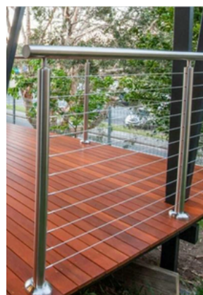
Deck Stainless Steel Cable Railing
